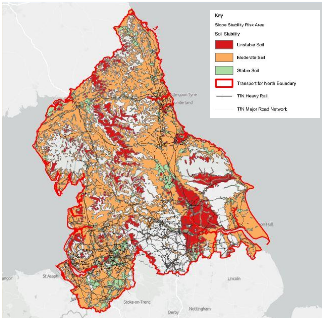
Figure 4.3: Slope failure risk areas across the TfN area
